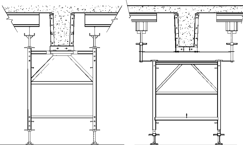
CONVENTIONAL LAYOUT
