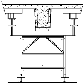
GARAGE BEAM
